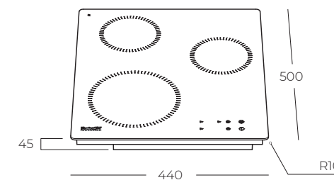
TM | cut-out for Top mount
