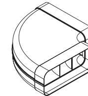
A700 D34 € 92 90° angular connection horizontal section 227 x 94 mm dimensions 288 x 288 x 94 mm
