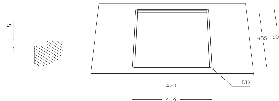
FT | cut-out for Flush-mount
