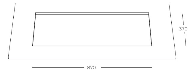
FT | cut-out for Flush-mount
