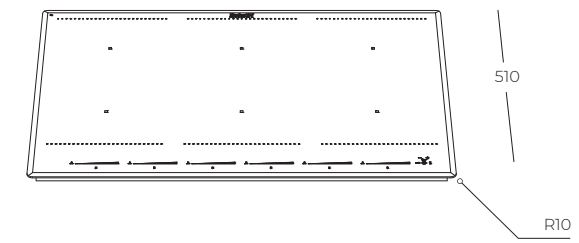
TM | cut-out for Top mount
