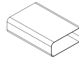
A700 D32 € 100 Rectangular tube section 222 x 89 mm dimensions 222 x 89 x 1000 mm
