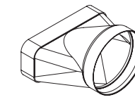
A700 D37 € 81 multi-section rectangular adapter 227 x 94 mm round Ø 148 mm dimensions 190 x 150 x 227 mm
