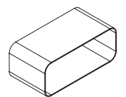
A700 D33 € 52 Angular connection section 227 x 94 mm dimensions 227 x 94 x 80 mm
