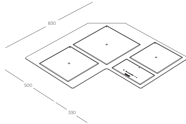
TM | cut-out for Top mount
