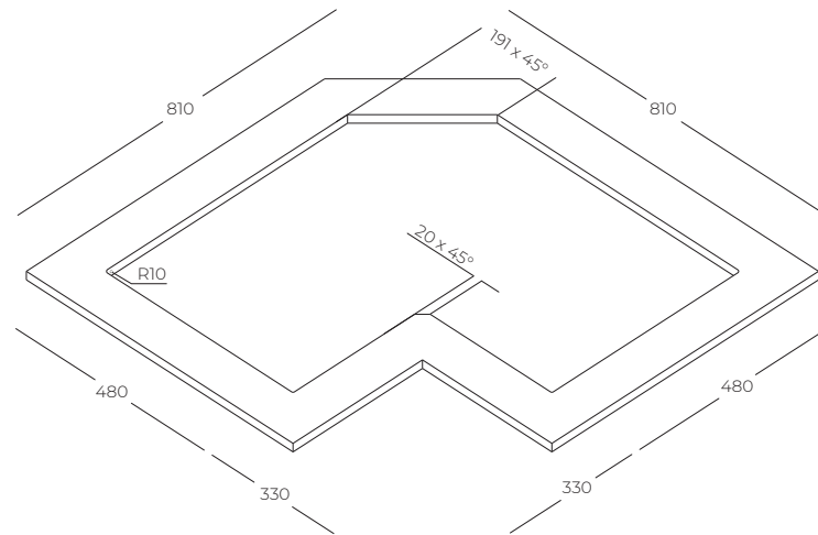
FT | cut-out for Flush-mount
