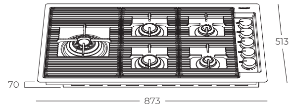
TM | cut-out for Top mount
