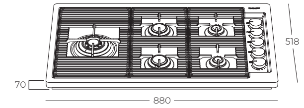
TM | cut-out for Top mount
