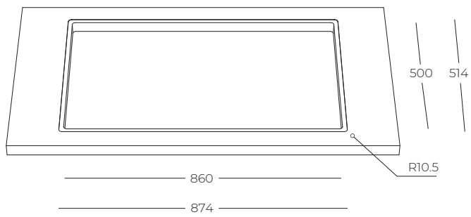
FT | cut-out for Flush-mount
